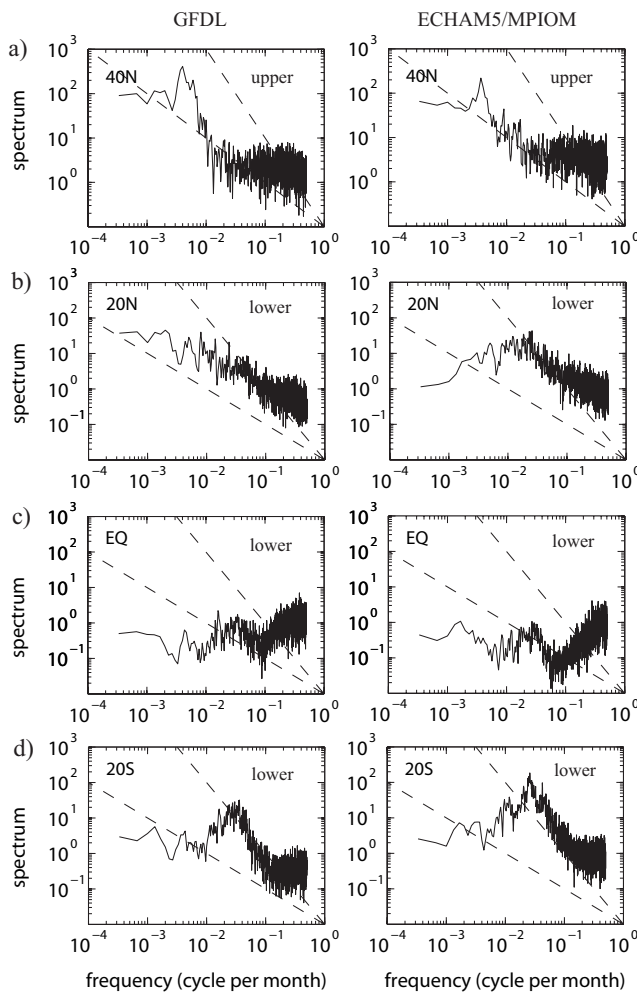
Figure 3. MOC Power spectra in the GFDL (left) and ECHAM5/MPIOM model (right): (a) 40N upper ocean (near 1200m), (b) 20N lower, (c) Equator lower, (d) 20S lower (lower ocean near 4000m). Dashed lines indicate spectral exponents \beta = 1 and 2 .
