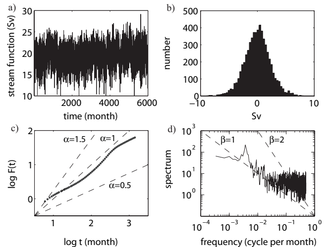
Figure 2. MOC at 40N in 1200m depth for the ECHAM5/MPIOM model: (a) time series, (b) anomaly frequency distribution, (c) fluctuation function by DFA2, (d) power-spectrum (5 overlapping windows). Dashed lines in (c, d) denote power-laws for exponents \alpha and \beta as indicated.
