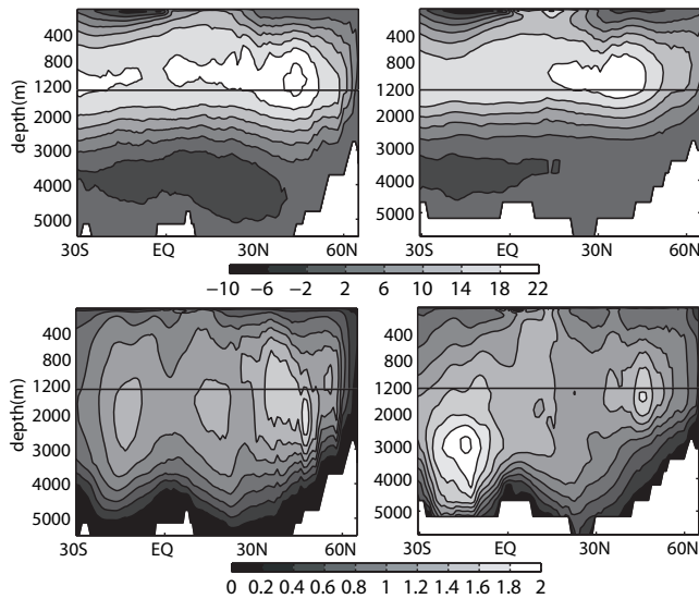
Figure 1. Mean (upper) and standard deviation (lower) of the zonally averaged streamfunction [Sv] in the Atlantic for the GFDL model (left) and ECHAM5/MPIOM (right).
