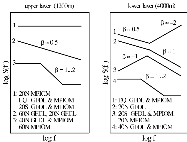
Figure 4. Sketch of main types of MOC power spectra found in the upper and lower level with ranges for the spectral exponent \beta . Locations of model spectra are indicated (see Figure 3).
