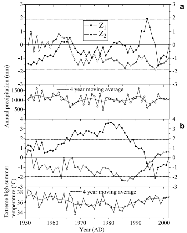
Fig. 6. Mann-Kendall analysis result of the annual precipitation (a) and that of the extreme high summer temperature (b) during 1950–2002 in the Yangtze Delta. The two dashed lines denote the 95% confidence level
