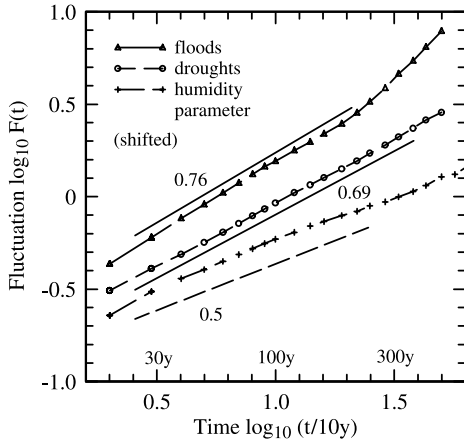
Fig. 7. Fluctuation functions F(t) for the decadal time scale t for floods ( \Delta ), droughts ( \circ ), and the humidity parameter ( + ) obtained by DFA. The lines describe power laws with exponents \alpha as indicated
