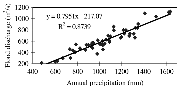
Fig. 4. Correlation between annual precipitation and the flood discharge during 1950–2002 at a tributary river basin of the Yangtze Delta
