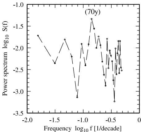
Fig. 8. Power spectrum S(f) for spectral frequency f of the maritime events with the maximum intensity at 70 years. S(f) is averaged in three non-overlapping segments of the total time series
