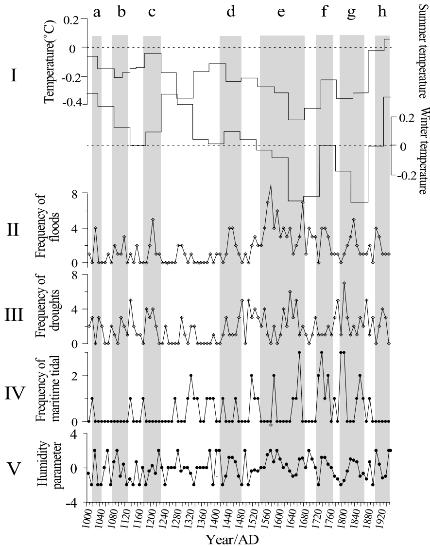
Fig. 2. Flood events, tidal events and temperature changes evolving in the Yangtze Delta. The dashed lines in panel IV and V denote the 50-year moving average, in panel I they denote zero degrees. The shaded zones mark periods of higher-frequency floods (the data are listed as the appendix) coinciding with climate changes of China (Wang et al., 2002)
