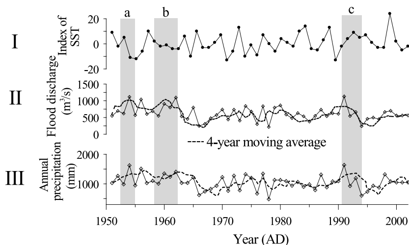
Fig. 3. Mean sea surface temperature (SST) index, flood discharge, and annual precipitation in the lower reaches of the Yangtze River from instrumental records (1950 to 2002); discharge with 4-year moving average (dashed) of rivers in the Yangtze Delta
