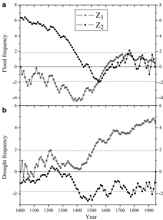
Fig. 5. Mann-Kendall analysis results of the flood frequency (a) and drought frequency (b) during 1000–1950 in the Yangtze Delta. The two dashed lines denote the 95% confidence level
